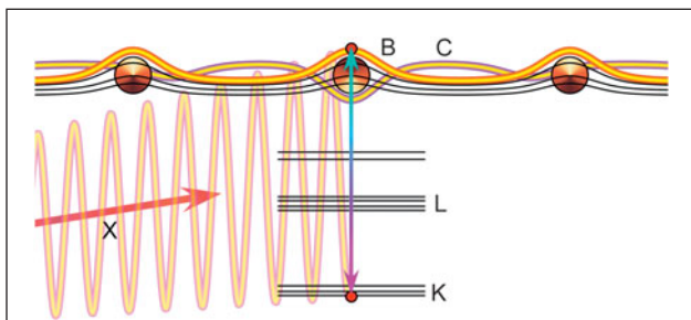
Figure 6. Schematic for the formation of an x-ray absorption fine structure. Absorption takes place by ejecting a core electron of the central atom from the K or L shell into the conduction band B or C, where it can travel to neighboring atoms and scatter back. The electron amplitude and energy levels depend minutely on the interference of these traveling waves, which depend on energy. Here, band state B has a slightly higher energy level than band state C at the central atom. The scattering process is a superposition of the absorption and stimulated emission of light, and lasts on a femtosecond scale. This process involves many attosecond cycles of the x-ray wave (X), during which a standing electron wave builds up, thus modulating the absorption probability. In quantum mechanics, the process of absorption is not localized at a fixed position, but instead is distributed over many equivalent atoms, giving rise to the interference.
