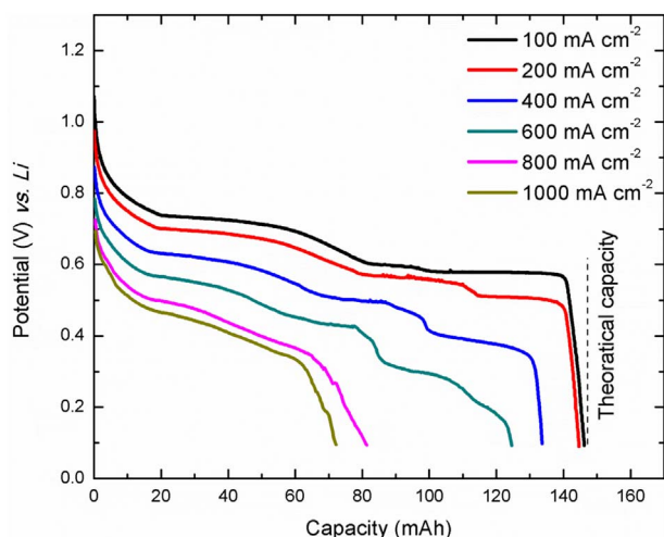
Fig. 7. The discharge potentials of 60:40mol% Bi-Sb alloy in the three-electrode cell at different current densities (range \sim 100 –1000 \text{mA cm}^{-2} ).
