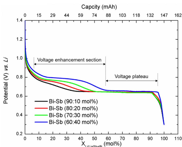
Fig. 1. The discharge curves of working electrodes in the three-electrode cell at the current density of 50 \text{ mA cm}^{-2} .
