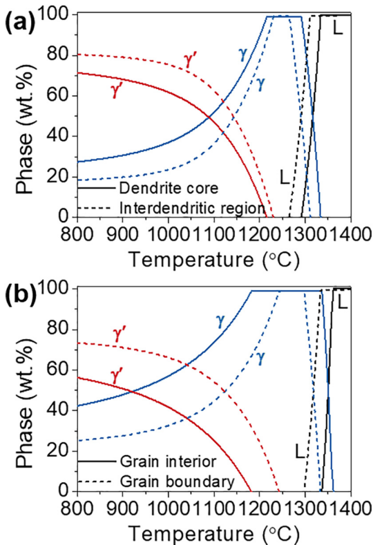
Fig. 8. Thermodynamic calculation of phase diagrams based on the chemical compositions of (a) the cladding layers and (b) the primary HAZ listed in Table 3, respectively.
